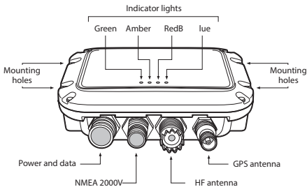
Figure 2 AIS transceiver overview
