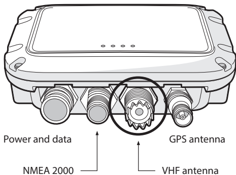
Figure 9 Position of the VHF antenna connector
