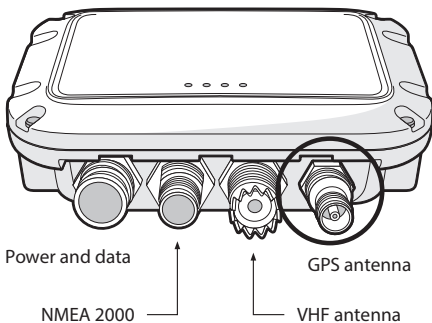
Figure 8 Position of the GPS antenna connector
