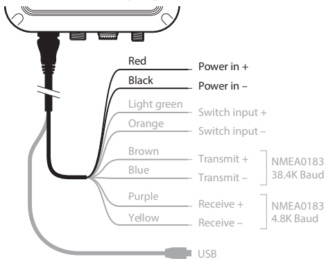
Figure 12 Connecting the power supply
