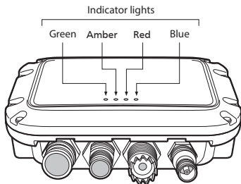
Figure 14 Indicator location on the AIS transceiver unit
