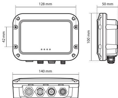
Figure 5 AIS transceiver dimensions
