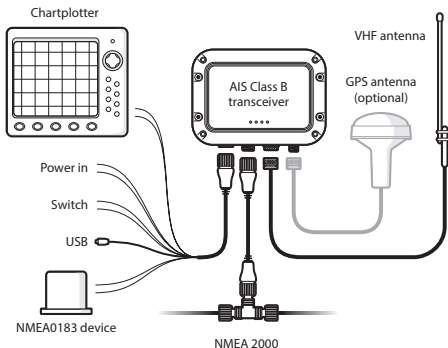
Figure 4 Typical installation configuration
