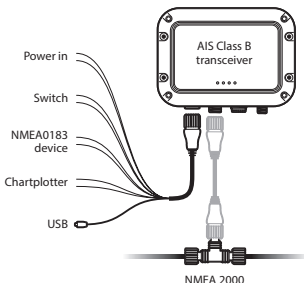
Figure 3 Electrical connections to the AIS transceiver
